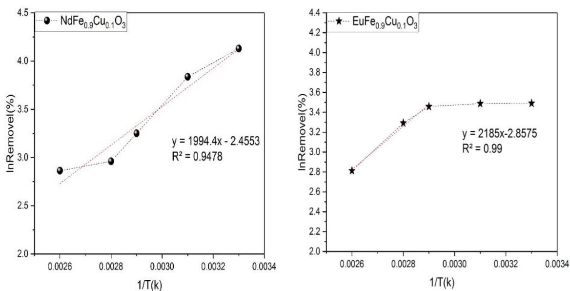
Figure 6. The Arrhenius plot of \ln R % vs 1/T . The time, volume, pH and concentration of dyes solutions are 150min, 50ml, 5.1 and 10ppm respectively.
